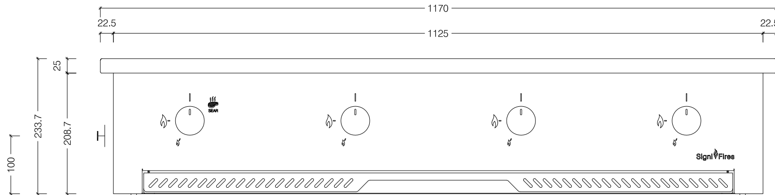
Front View
