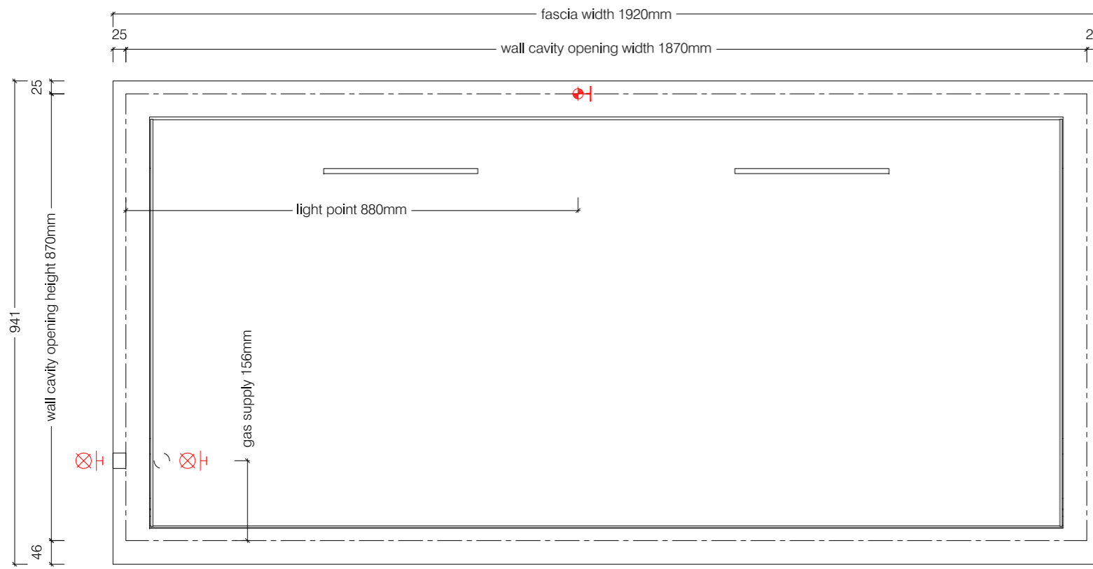
Front View
