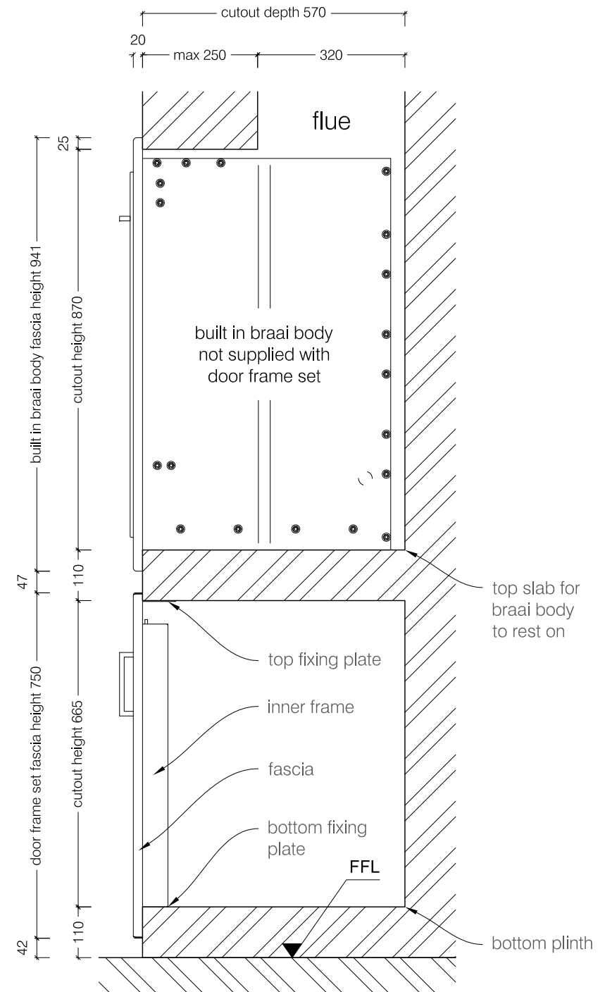
Side View
