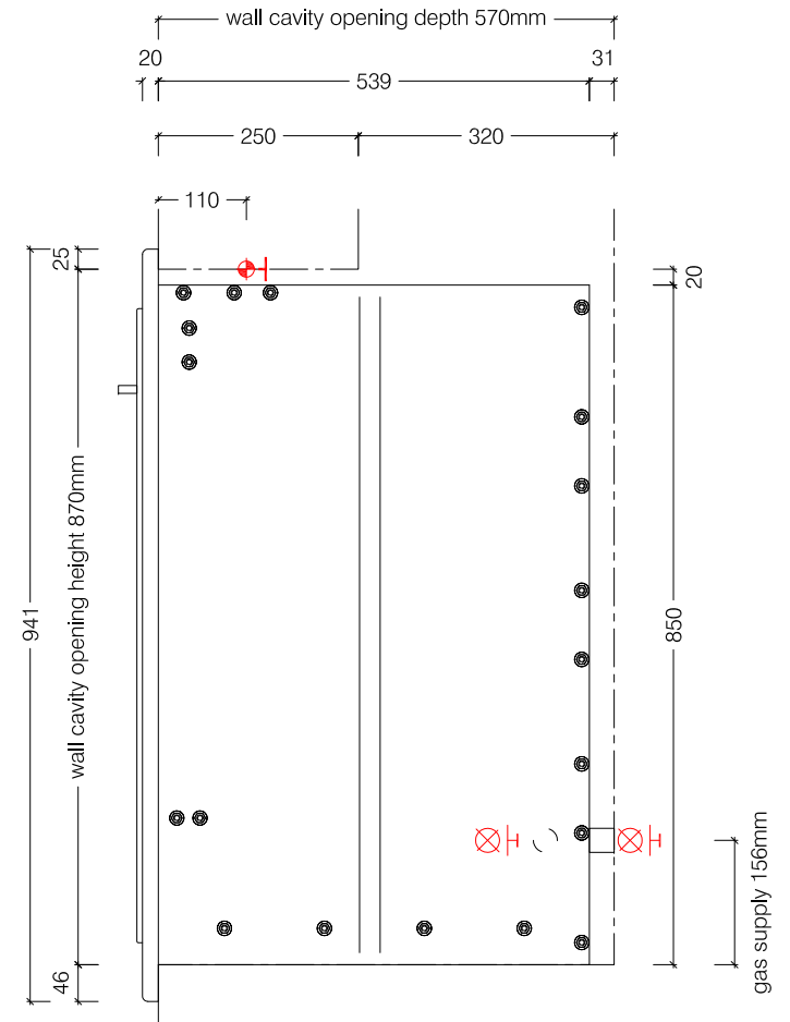
Side View
