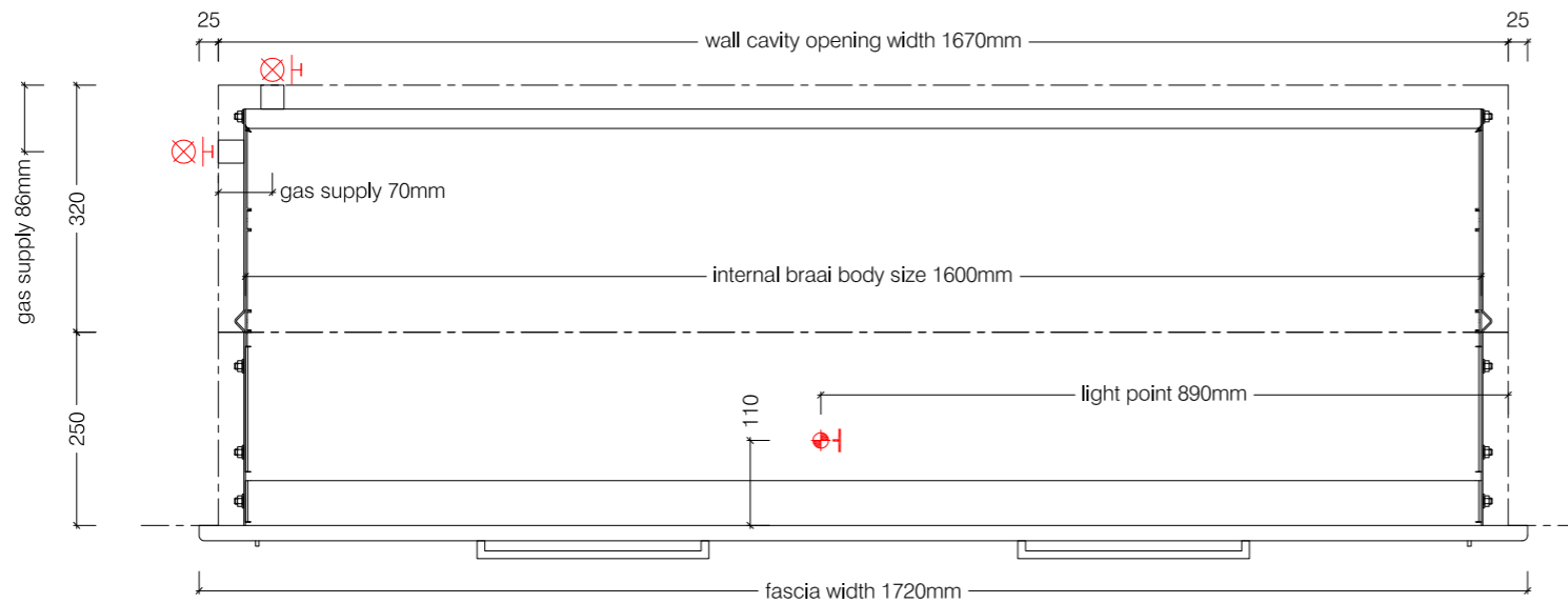
Top View
