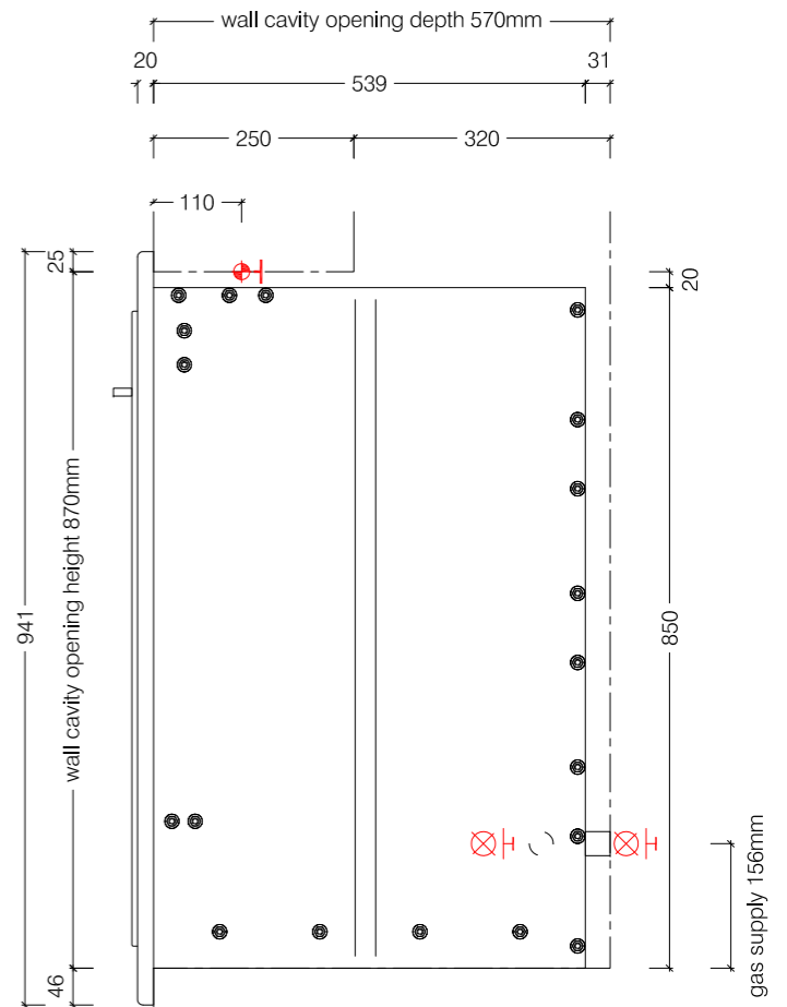
Side View
