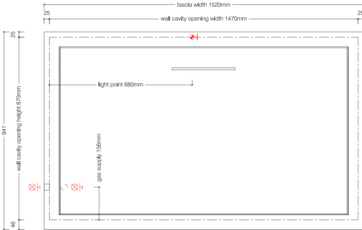
Front View
