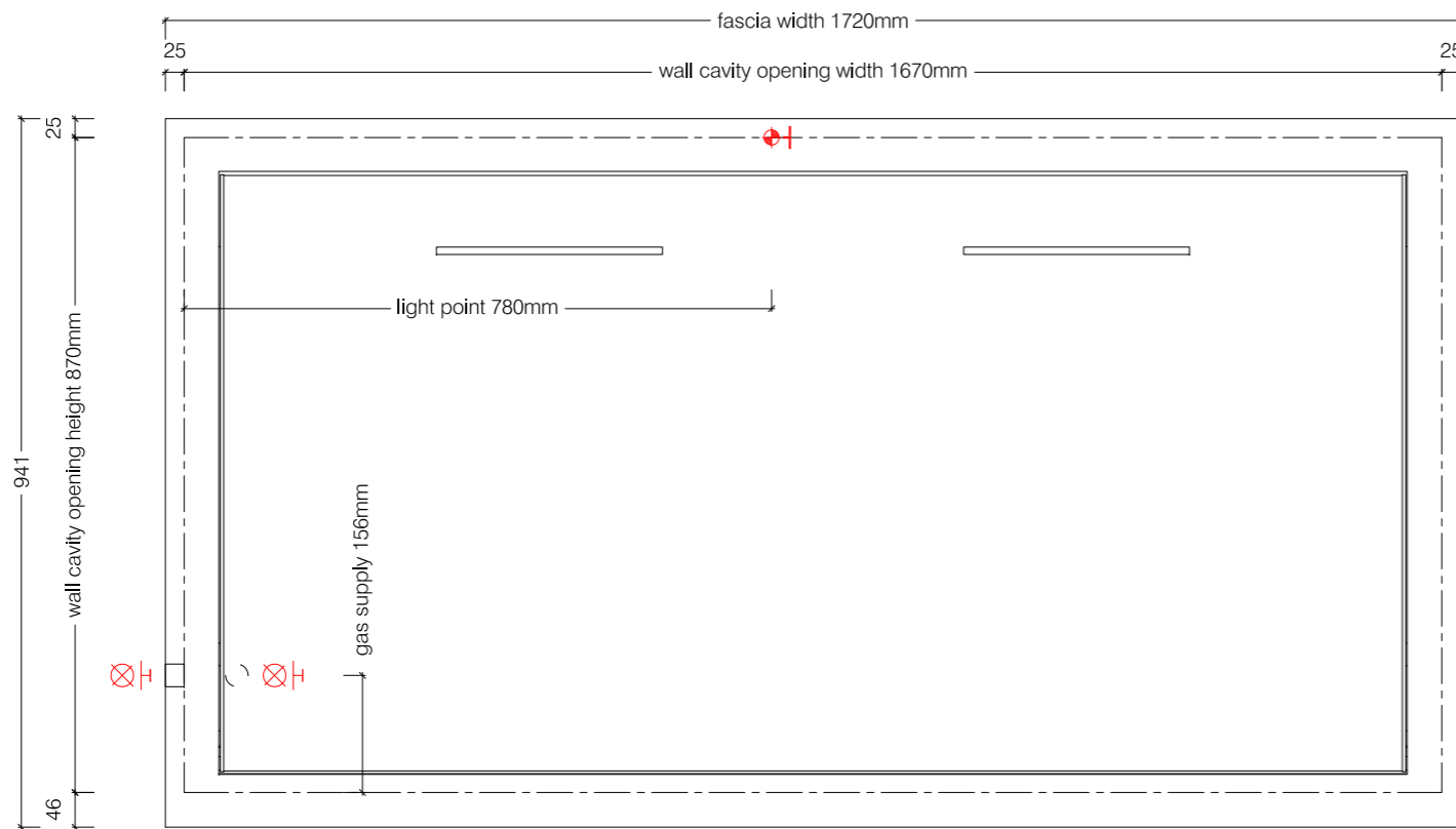
Front View
