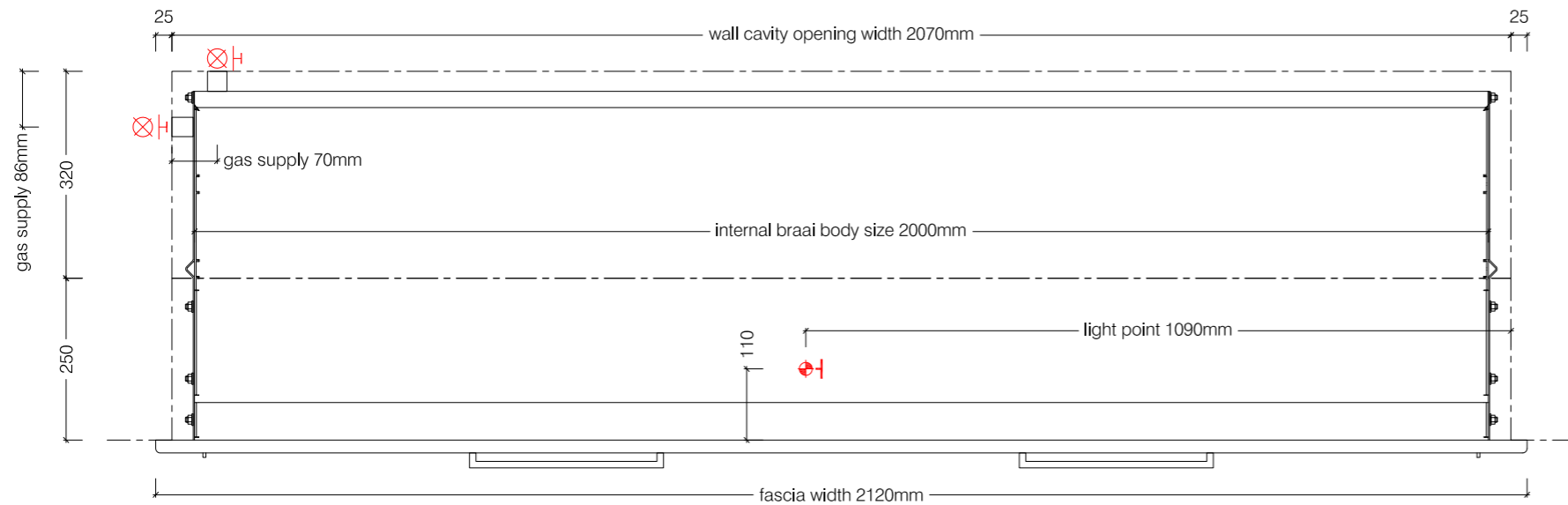
Top View
