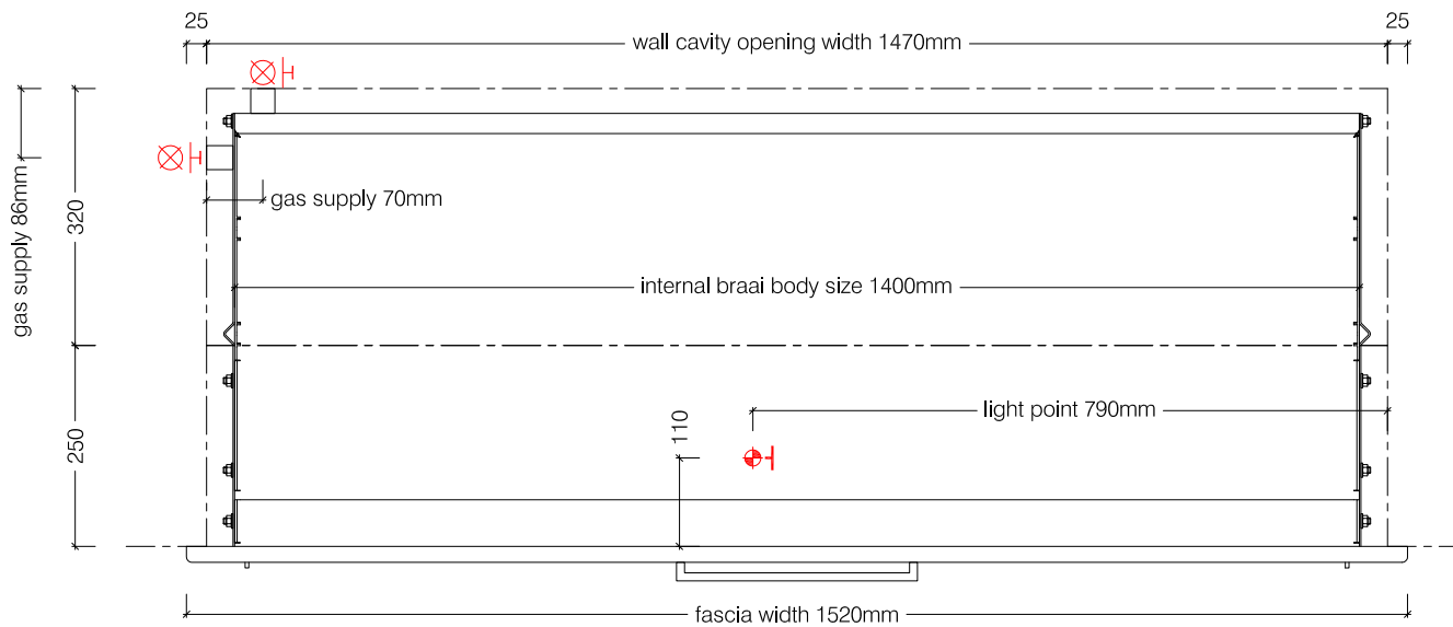
Top View
