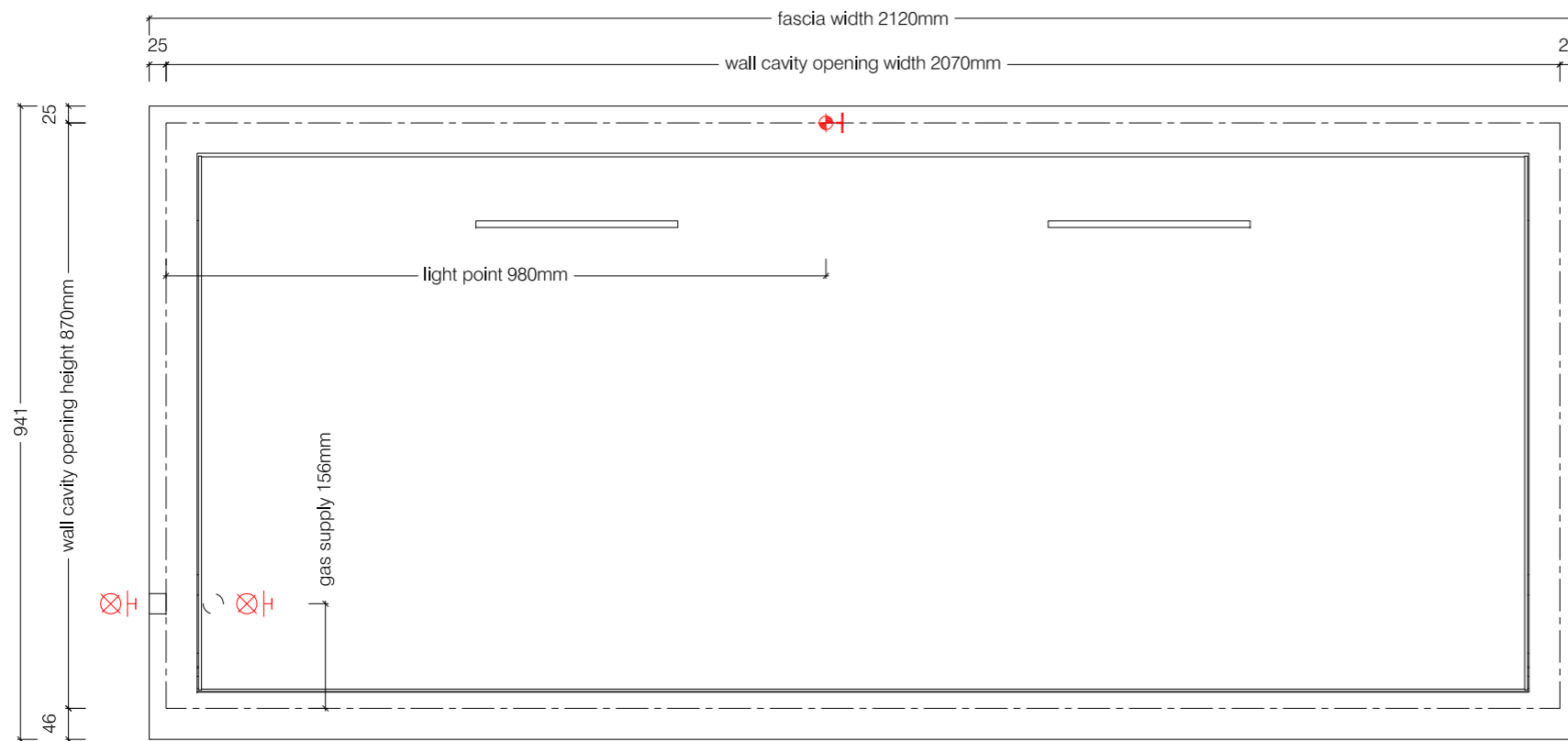
Front View
