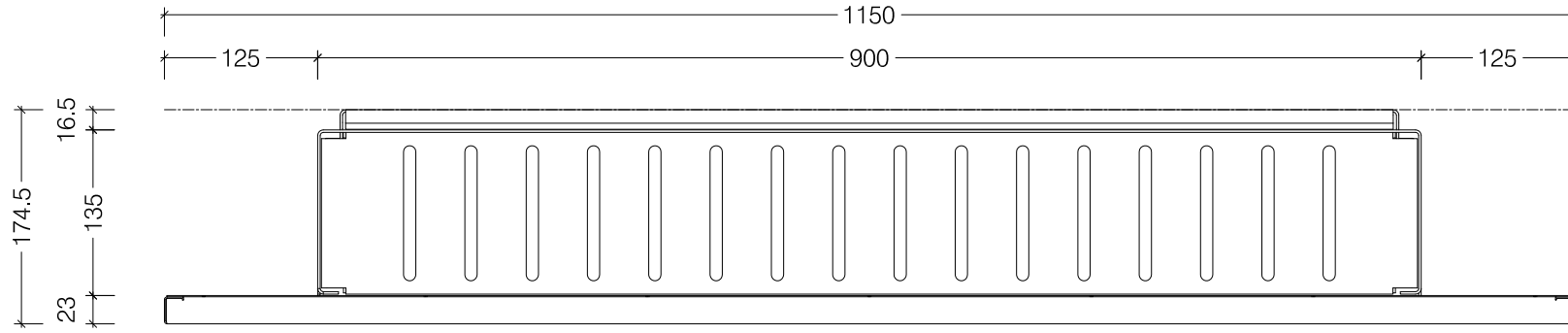
Top View
