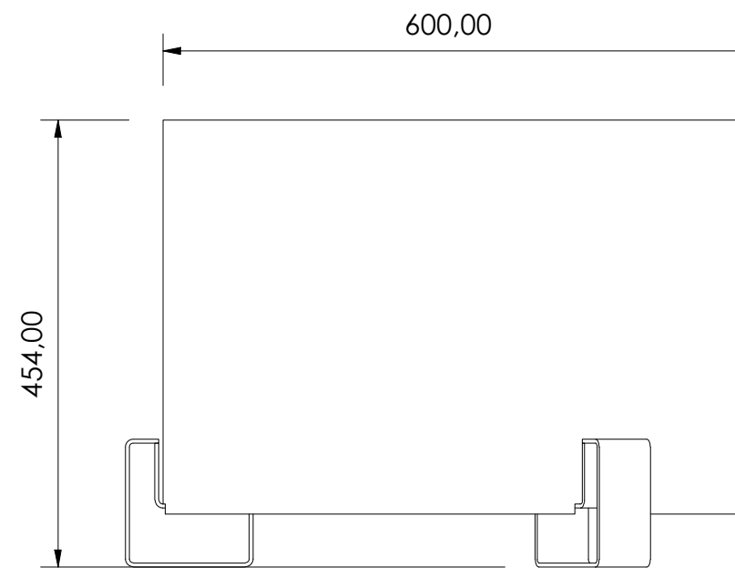
View ( 1 : 7 )
