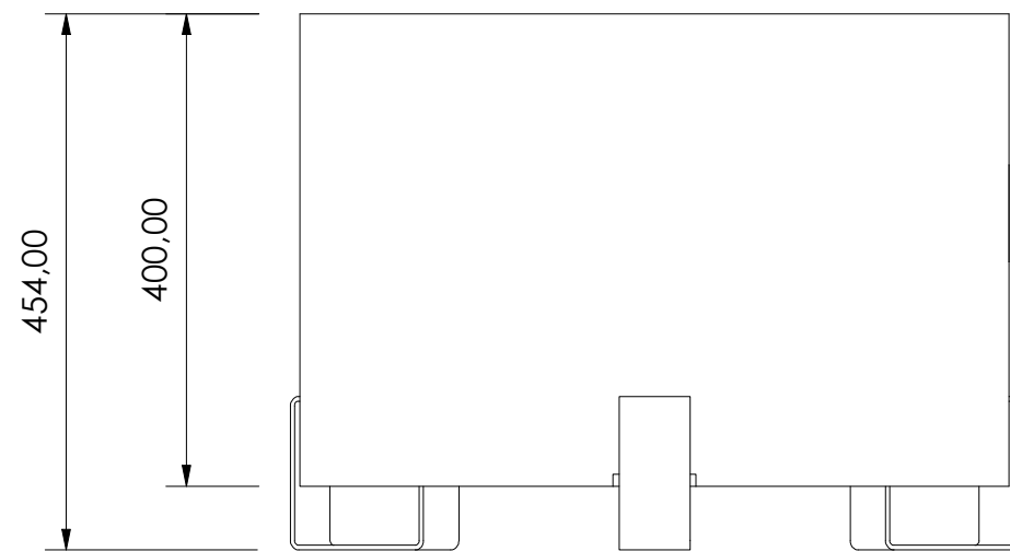
View ( 1 : 7 )
