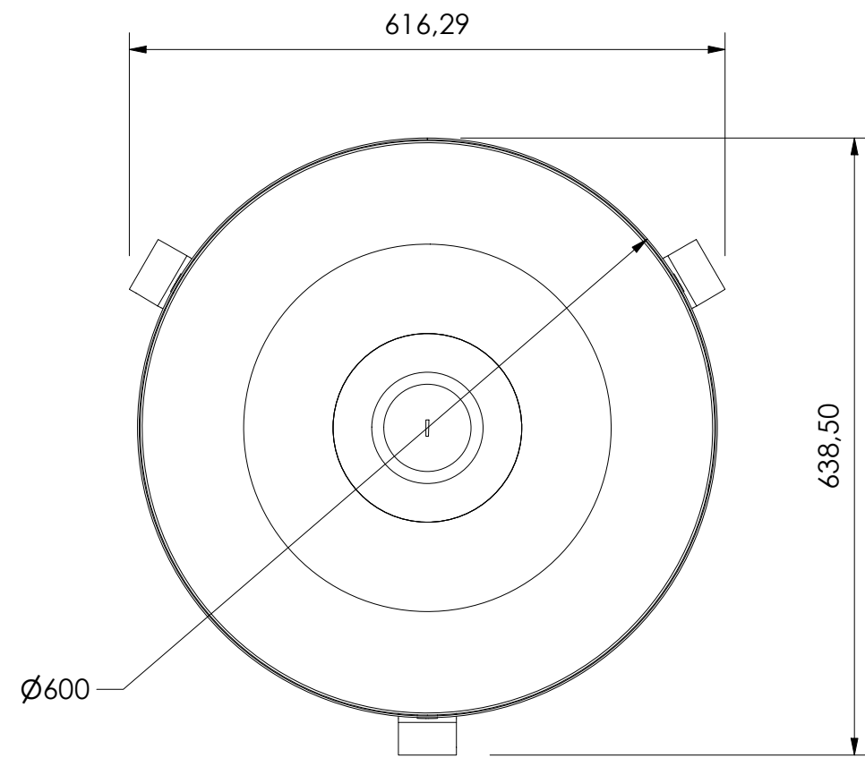
View ( 1 : 7 )
