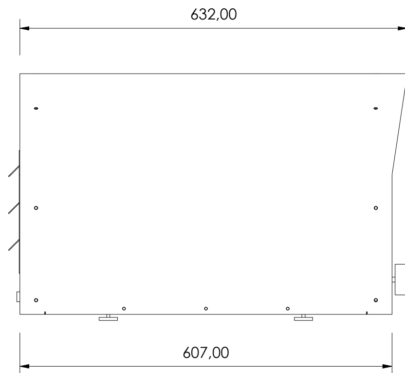
View ( 1 : 6 )
