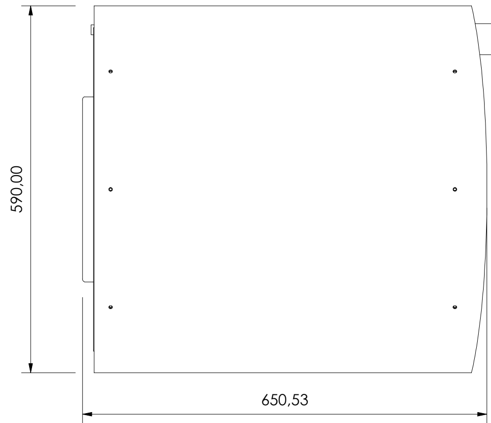
View ( 1 : 6 )
