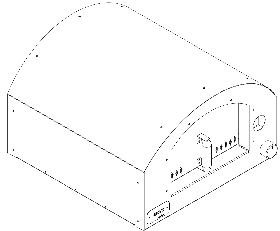
View ( 1 : 6 )
