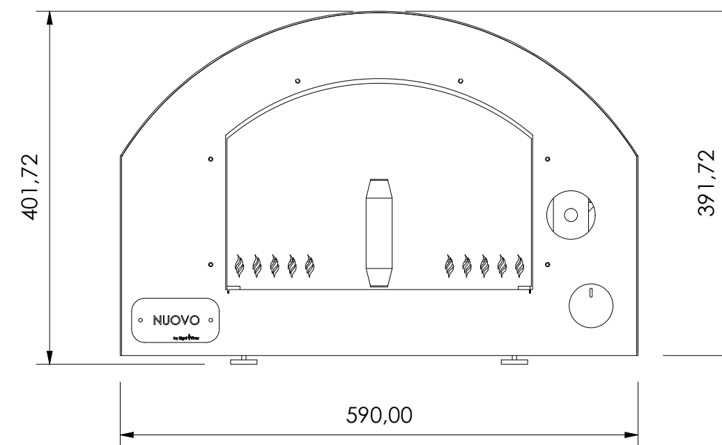
View ( 1 : 6 )
